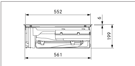
Fig. 3.5 Vista frontal PURSU
