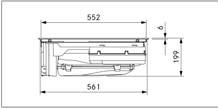
Fig. 3.2 Vista frontal PURSA
