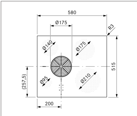
Fig. 3.4 Vista superior PURSU
