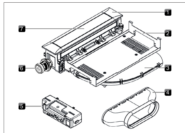
Fig. 3.5 Emfang PKA3/PKA3AB
