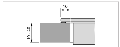
Fig. 9.13 Overlay dimensions for surface mounting
