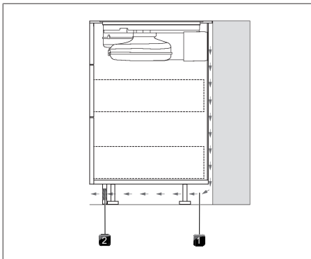
Fig. 9.23 Return flow aperture in the plinth area
