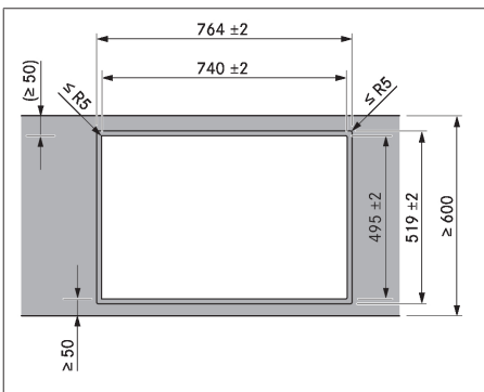
Fig. 9.10 Cut-out dimensions for flush installation
