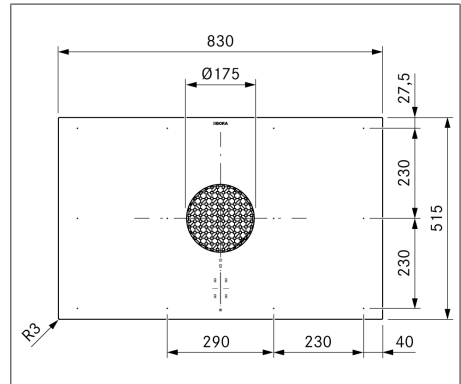
Fig. 3.1 PUXA appliance dimensions top view
