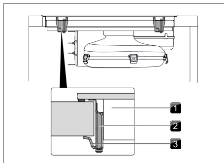
Fig. 9.35 Securing the cooktop in the middle
