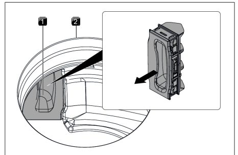
Fig. 7.5 Removing the filter replacement cover
