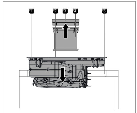
Fig. 9.18 Positioning the cooktop in the centre
