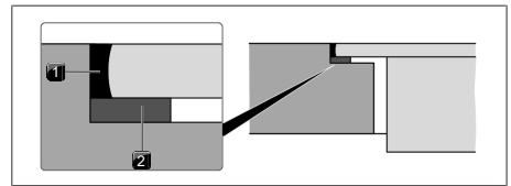
Fig. 9.28 Sealing tape in the case of flush installation
