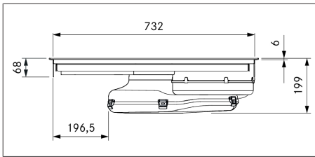
Fig. 3.8 PURA appliance dimensions front view
