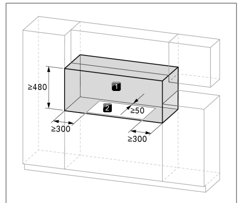
Fig. 9.3 Required clearance
