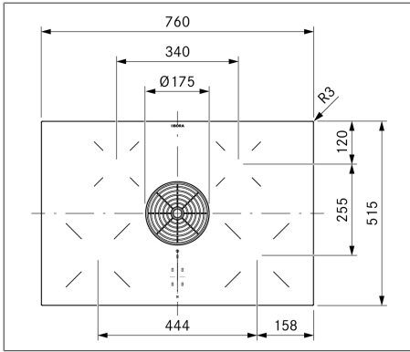
Fig. 3.7 PURA appliance dimensions top view
