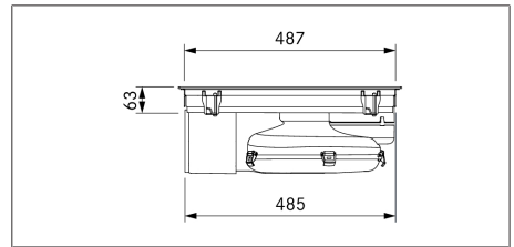
Fig. 3.12 PURU appliance dimensions side view
