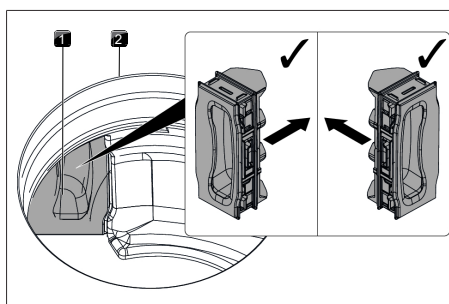
Fig. 7.11 Inserting the filter replacement cover
