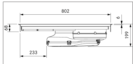
Fig. 3.2 PUXA appliance dimensions front view
