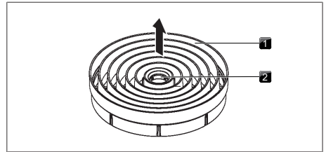
Fig. 7.2 Removing air inlet nozzle PURA, PURU
