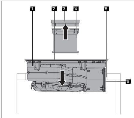
Fig. 9.32 Positioning the cooktop in the centre
