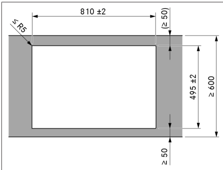
Fig. 9.8 Cut-out dimensions for surface mounting
