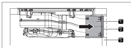
Fig. 9.36 Making a connection with the back panel
