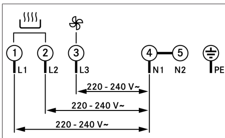
Fig. 9.43 Connection diagram for 3-phase connection
