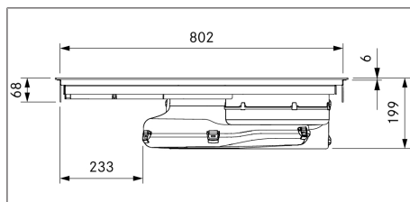
Fig. 3.5 PUXU appliance dimensions front view
