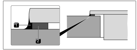
Fig. 9.27 Sealing tape in the case of surface mounting
