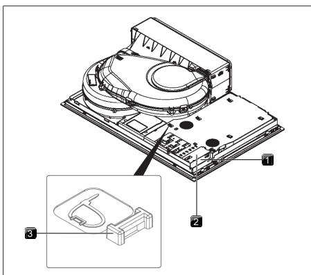
Fig. 9.46 Electrical connections of the cooktop
