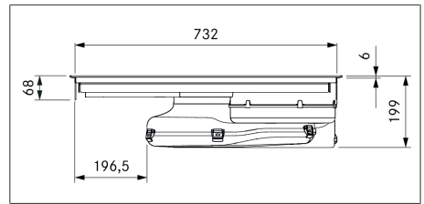
Fig. 3.11 PURU appliance dimensions front view
