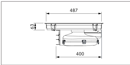
Fig. 3.9 PURA appliance dimensions side view
