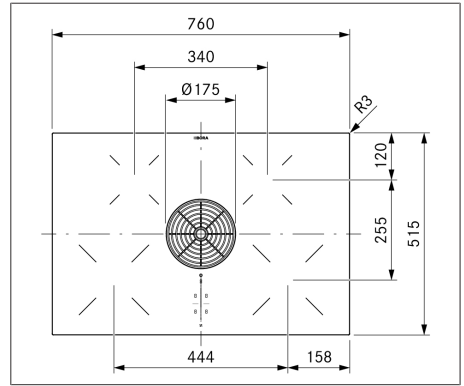
Fig. 3.10 PURU appliance dimensions top view
