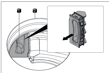
Fig. 9.37 Remove the filter replacement cover
