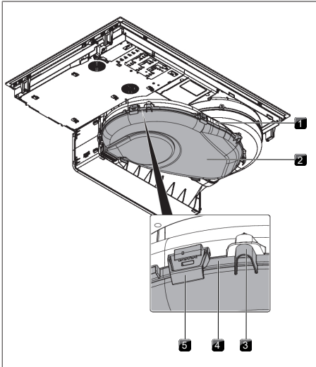
Fig. 7.4 Air guiding housing
