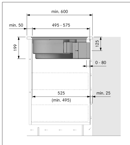
Fig. 9.24 Installation dimensions in the case of recirculated air, installation variant A
