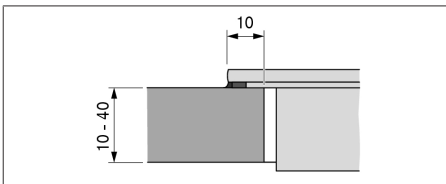
Fig. 9.9 Overlay dimensions for surface mounting
