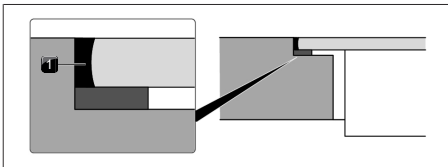
Fig. 9.52 Silicone sealant for flush installation
