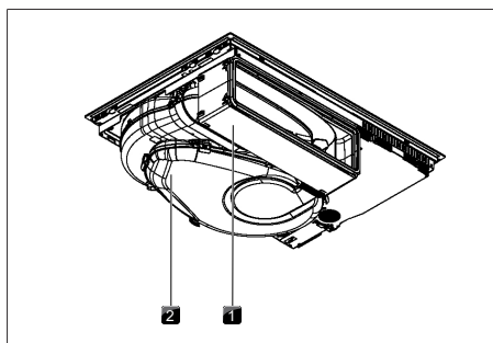
Fig. 4.3 Rear view of PUXU, PURU
