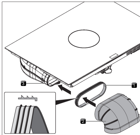
Fig. 9.22 Connecting the duct system
