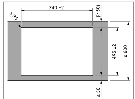
Fig. 9.12 Cut-out dimensions for surface mounting
