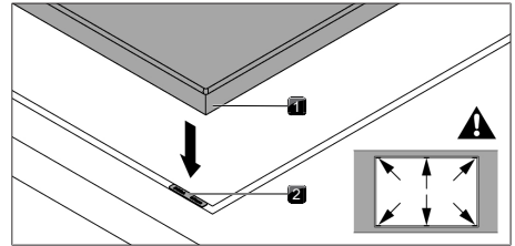
Fig. 9.33 Positioning the height adjustment plates
