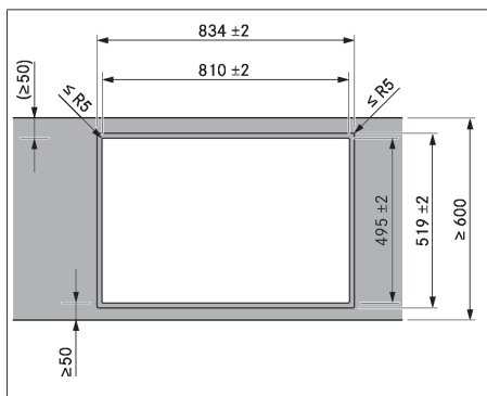
Fig. 9.6 Cut-out dimensions for flush installation
