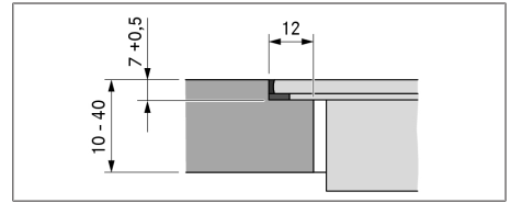
Fig. 9.11 Rebate dimensions for flush installation
