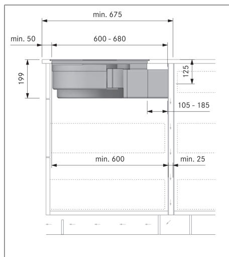
Fig. 9.30 Installation dimensions for recirculation installation variant A, depth of worktop 675 mm and over
