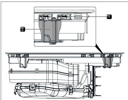
Fig. 9.17 Fitting the installation clamps
