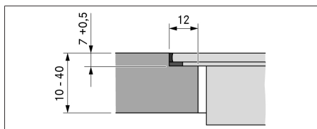
Fig. 9.7 Rebate dimensions for flush installation
