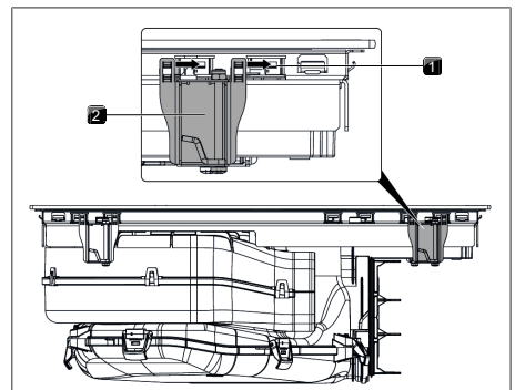
Fig. 9.29 Fitting the installation clamps
