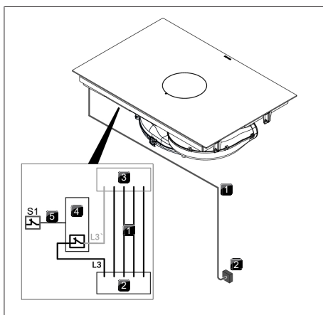
Fig. 9.42 Connection diagram with external switch contact
